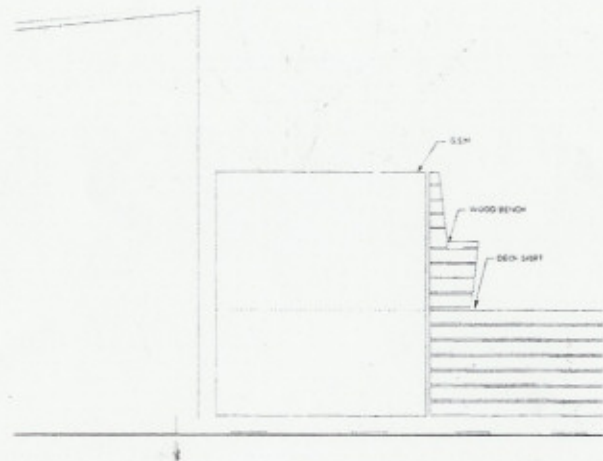
C1 G-PLANT AND BENCH NORTH ELEVATION 3/4"=1'-0"
